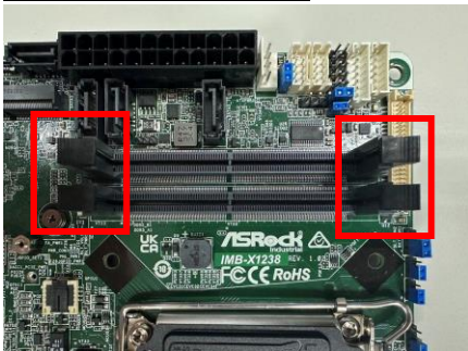
Original DIMM socket
